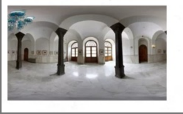
Virtual tours
