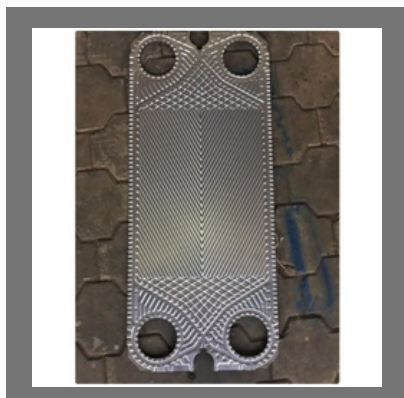
Alfa Laval M10M Plate Heat Exchanger
