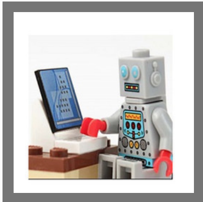
Chatbots Service
