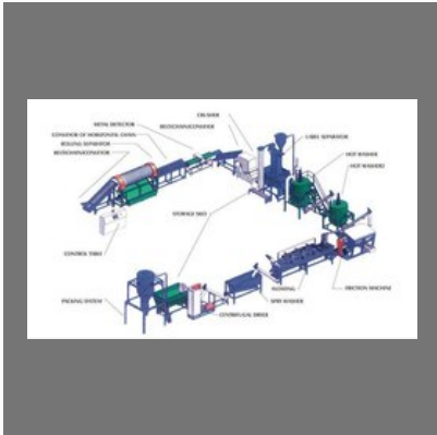
Pet Flake Washing Plant
