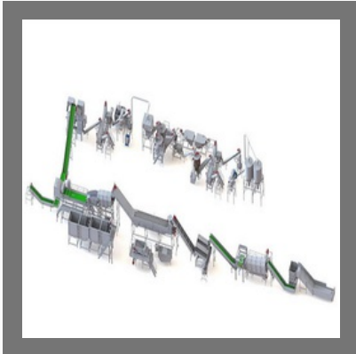
Recycled PET Bottle Flake Plant
