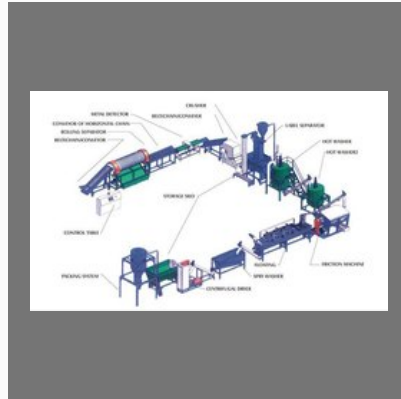
Pet Flake Washing Line
