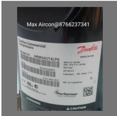
HRM042U1LP6 Danfoss Scroll Compressors
