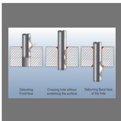
Automatic Machine Hole Deburring Tools
