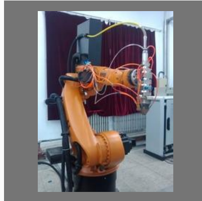
ABB Robot Laser Cladding Machine
