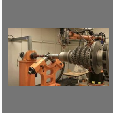
Robot Laser Cladding Machine
