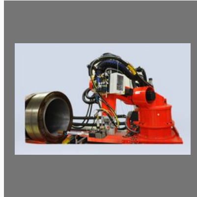
Laser Hardening Machine
