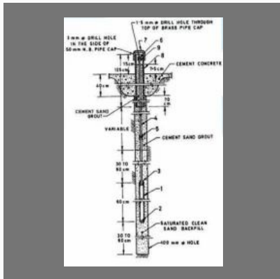
Porous Tube Piezometers
