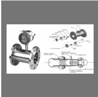
Turbine Flow Meter
