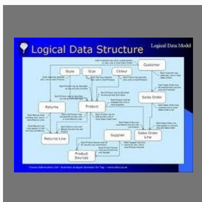
Data Structure
