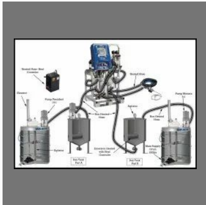
Hydraulic Connection Schematic Line Diagram
