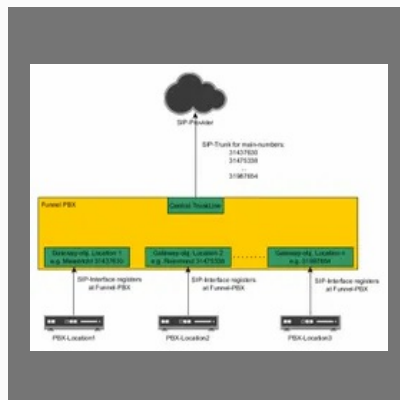
SIP Central
