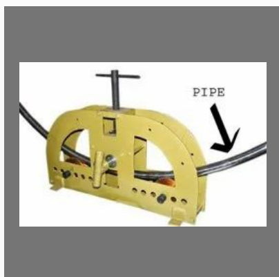
Pipe Bending Machine
