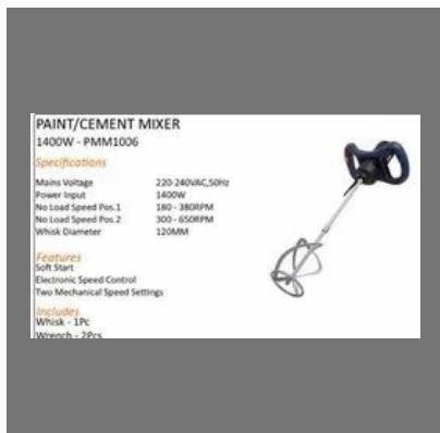
CEMENT MIXER
