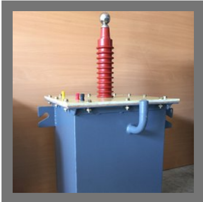
30kV 100mA High Voltage Transformer
