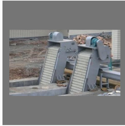
Mechanical Screen Bar
