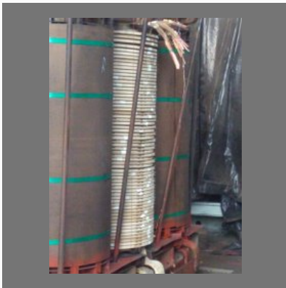
New HT Disc Type Coil With LV Fitted In 3,500 Kva Kirloskar Transformer
