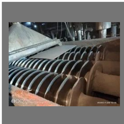
Screw Conveyor hollow flight
