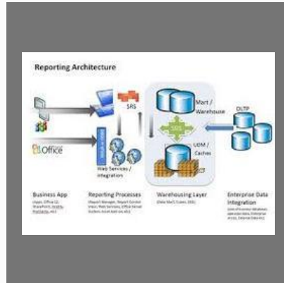
Enterprise Reporting
