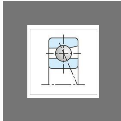
Single Row Angular Contact Ball Bearing
