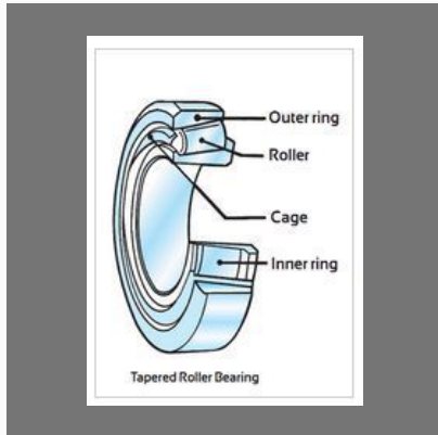
Single Row (TRB) Bearing
