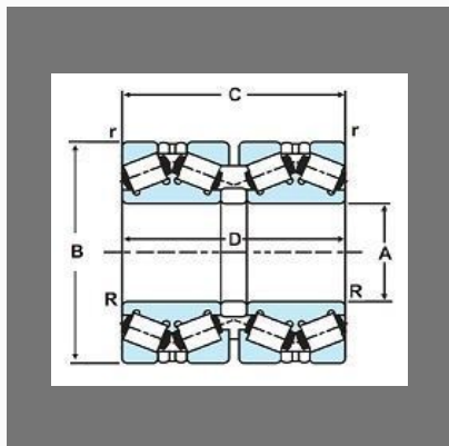
Four Row Tapered Roller Bearing (TRB)
