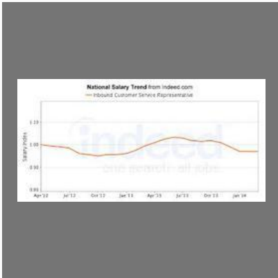
Inbound-Customer-Services
