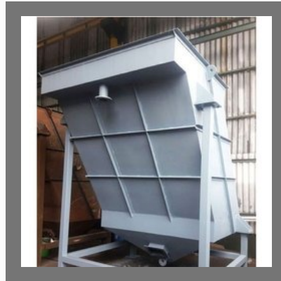
Parallel Plate Lamella Clarifier
