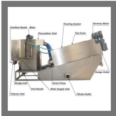
Volute Sludge Dewatering Machine
