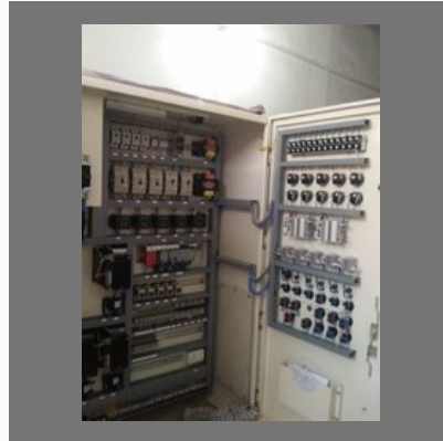
Slipring Motor Starter
