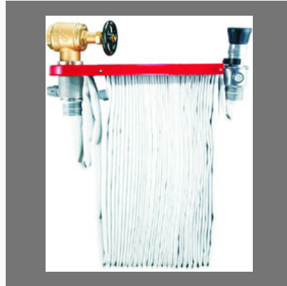
Hose Rack Assembly
