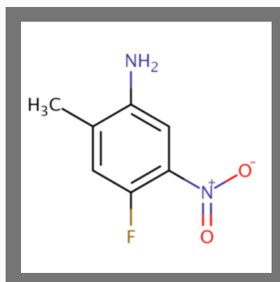
2-Methyl-5-Nitroaniline
