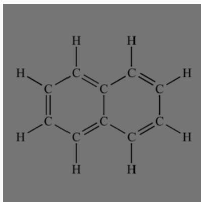
Naphthalene Chemical
