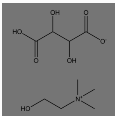
Choline Bitartrate
