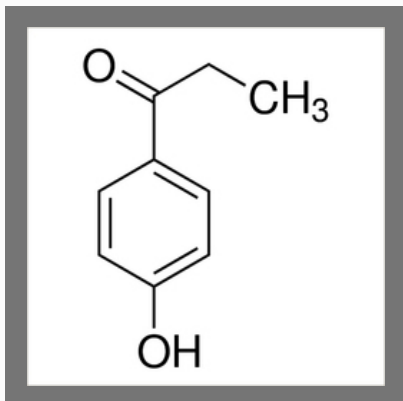
4-Hydroxy Propiophenone
