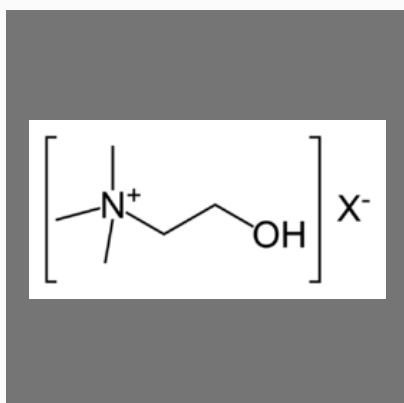
Choline Base
