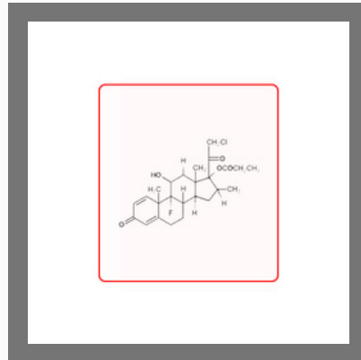
Clobetasol Salts
