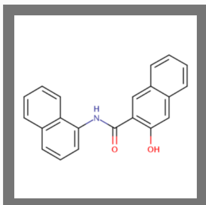
3-Hydroxy-2-Naphthilide
