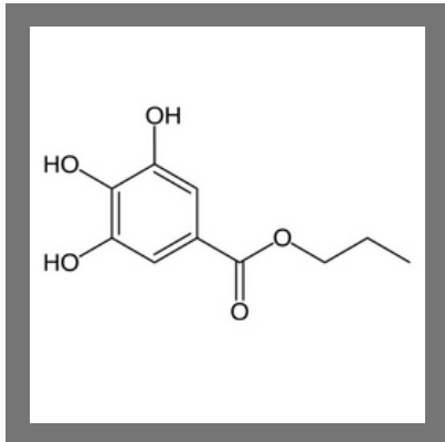
Propyl Gallate
