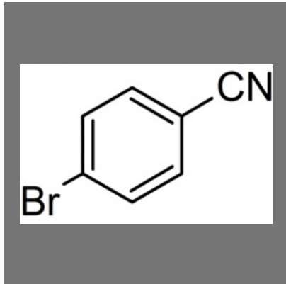
2 / 3 / 4 - Bromobenzonitrile
