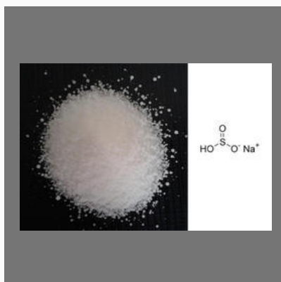
Sodium Bisulphite
