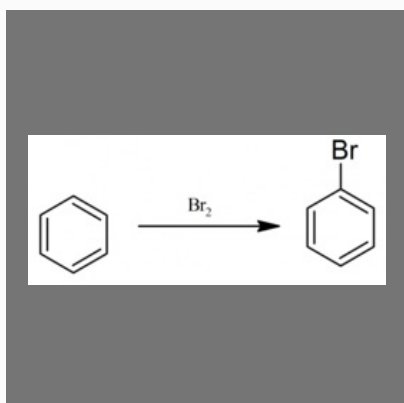
Bromobenzene
