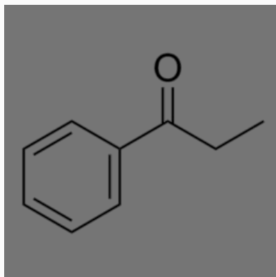
Propiophenone
