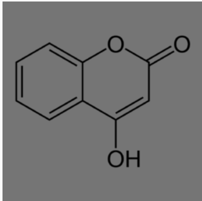
4 Hydroxycoumarin
