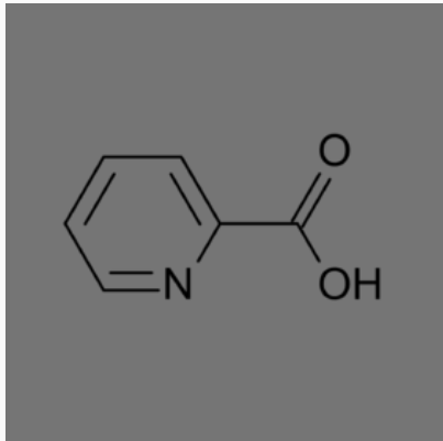
Picolinic Acid
