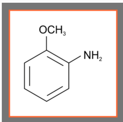
Ortho Anisidine
