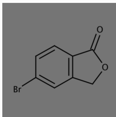
5-Bromophthalide
