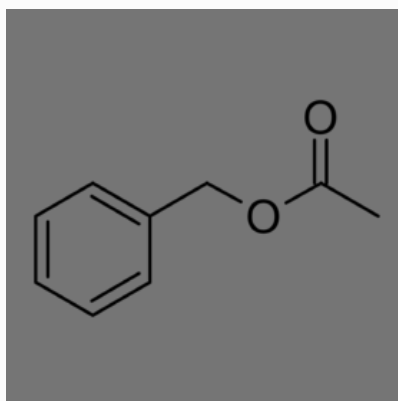
Benzyl Acetate
