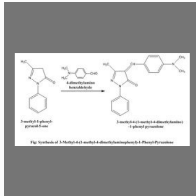
Pyrazolones Series
