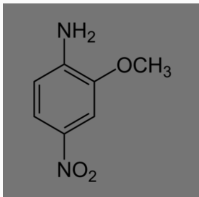
2-Methoxy-4-Nitroaniline
