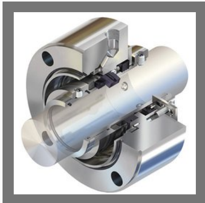
Pump Sealing
