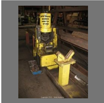
Hydraulic Angle Cutting and Shearing machine
