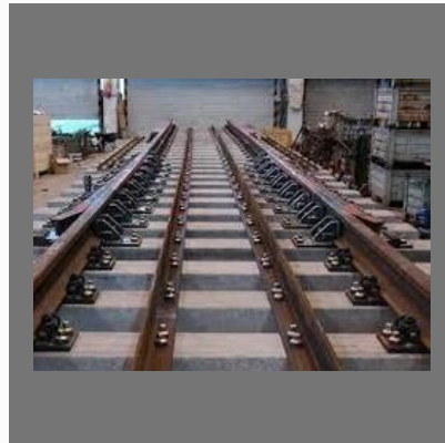
Switch Expansion Joints
