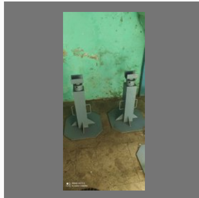
Cable Drum Screw Jacks 2 Ton
