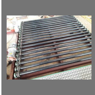
Powered Roller Conveyor
