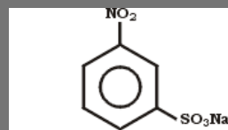
STRUCTURAL FORMULA
