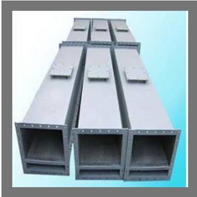
Air Slides
