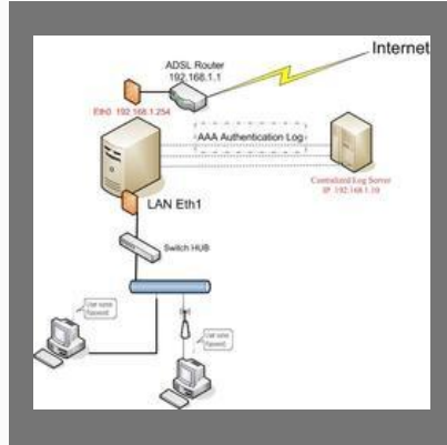
NAT - SYSLOG Server , IP Log Server , IP Syslog
