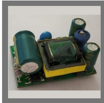
IOT 10W (5V/2A) SMPS Power Supply
