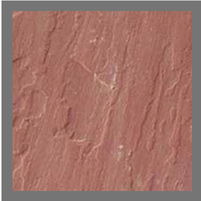
Mandana Stone
