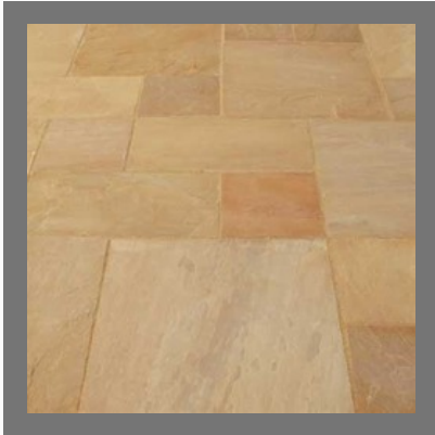
Natural Sandstone
