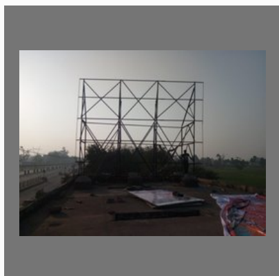
Unipole Structure
