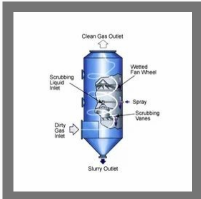
Wet Scrubber
