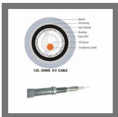
H.F Co-Axial Cables
