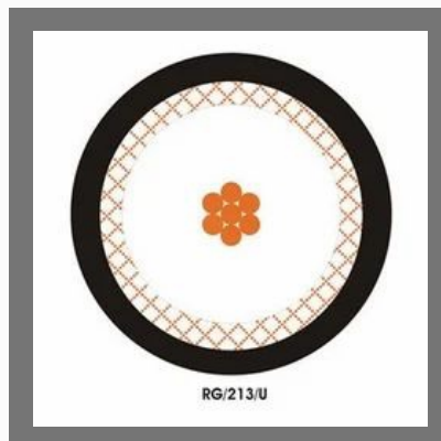
R.F Co-Axial Cables
