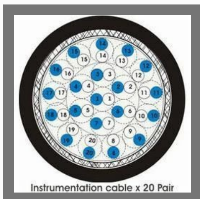
Instrumentation Cables
