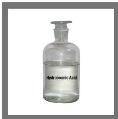
Hydrobromic Acid
