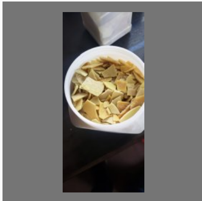
Sodium Hydrosulphide
