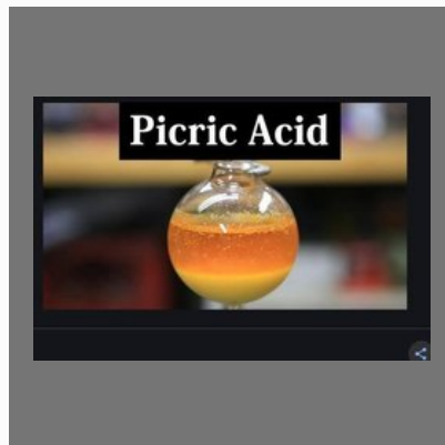
Picric Acid
