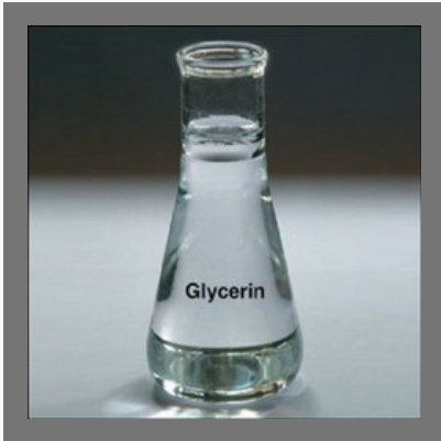
Liquid Glycerine
