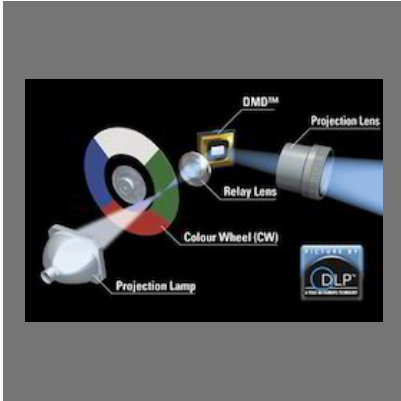
Multimedia Projectors
