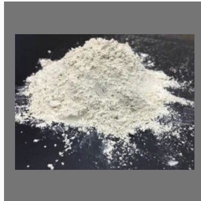
Zeolite Powder
