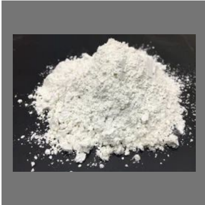
Pyrophyllite Powder
