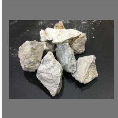
Calcined Pyrophyllite
