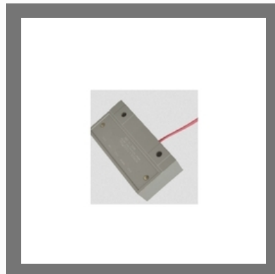
Pepperl & Fuchs 20FR1-6B 61 mm Magnetic Field Sensor
