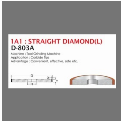
Straight Diamond Wheels
