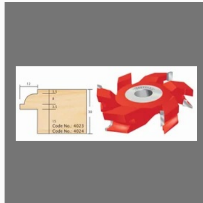
Rebating Cum Molem Cutter
