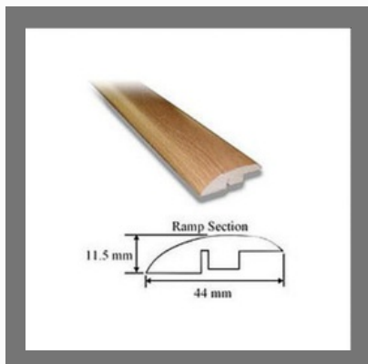
T Bar Profile
