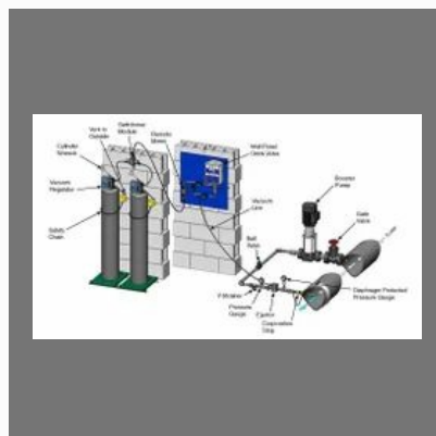
Gas Chlorination System
