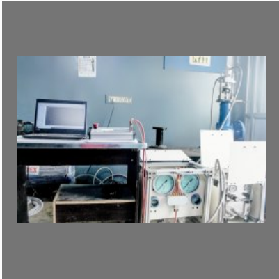
Online Hydraulic Kit
