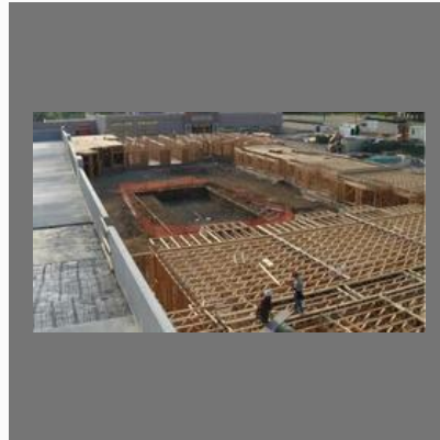
Swimming Pools Construction
