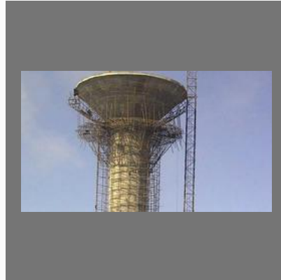
RCC Elevated Twin Service Reservoir
