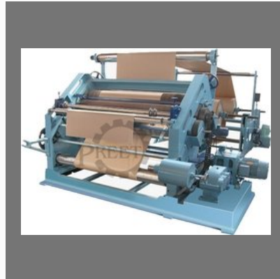
Vertical Paper Corrugating Machine
