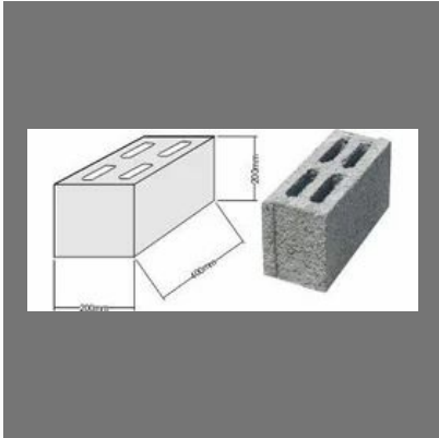
Hollow Blocks
