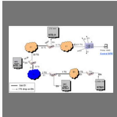
Network Diagram/Remote Device Management
