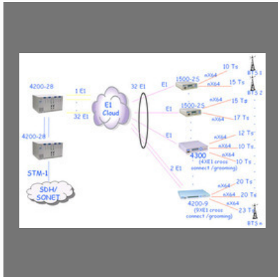
32E1 Cross-connect
