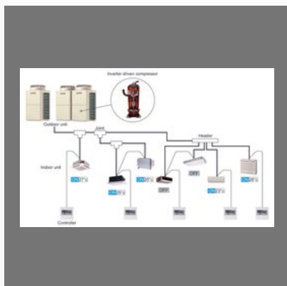
VRF System
