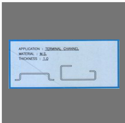
Terminal Channel
